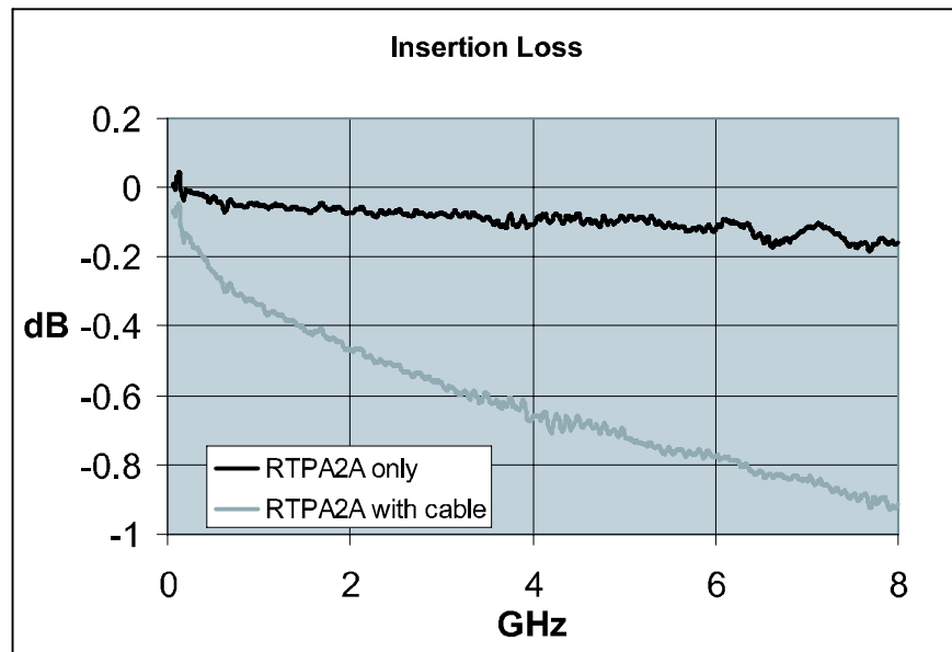
Figure 10: Insertion loss
